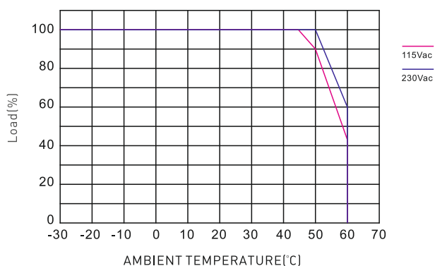
Temperature load curve
